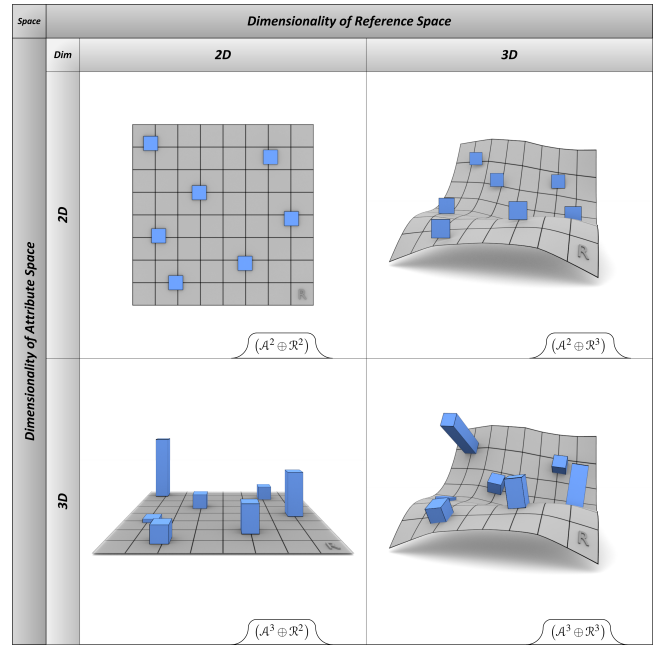
Figure 1: Systematization of visualization techniques based on the dimensionality of the attribute space’s and reference space’s presentation ( \mathcal{A} and \mathcal{R} respectively). For simplicity and clarity, the visual variables of the attribute representations are limited to a single color (blue) and a single item shape (square).
