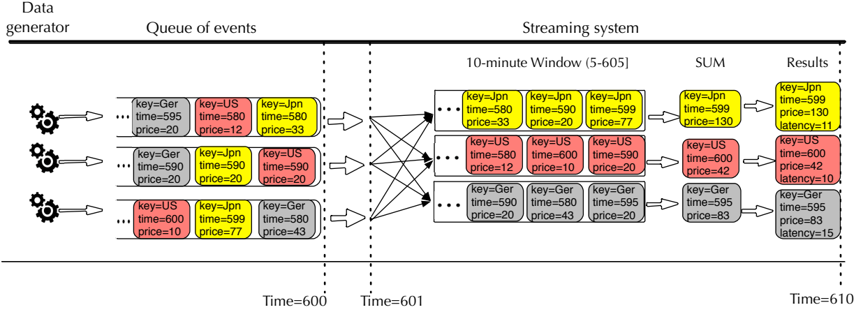
Fig. 1: End-to-end example of an aggregation query. The data generator produces tuples on a given event-time (before t_{\text{time}}=600 ), a second later the events enter the streaming system where they are grouped by their key, and finally aggregated (SUM). The event-time latency of the output tuple equals to the maximum event-time latency of elements in each window.
