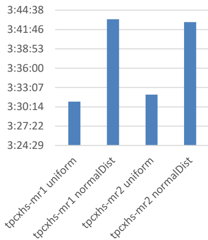
Figure 5: HSSort wall clock time
