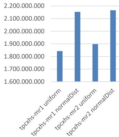
Figure 6: HSSort CPU time
