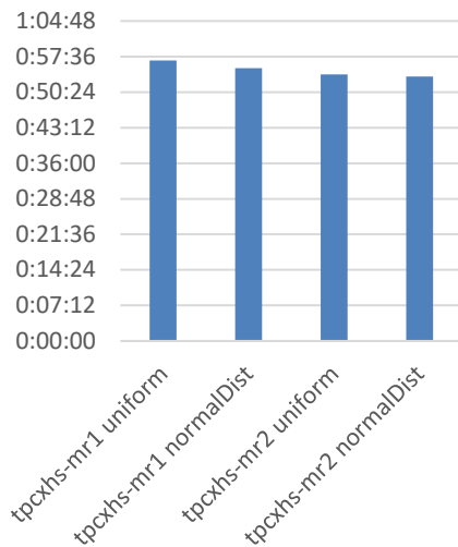
Figure 3: HSGen wall clock time
