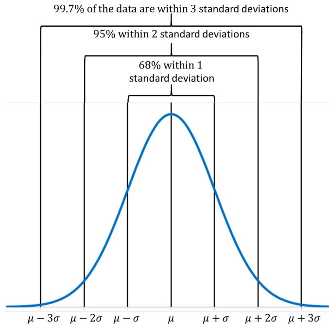
Figure 1: Normal distribution, its parameters and their implications 2
