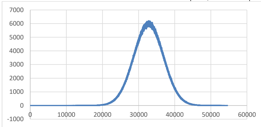
Figure 2: Accumulated density with mu: 2^{79} sigma: 2^{76} quantized from highest 16 bit of the full 80 bit value to mu: 32768 and sigma: 4096
