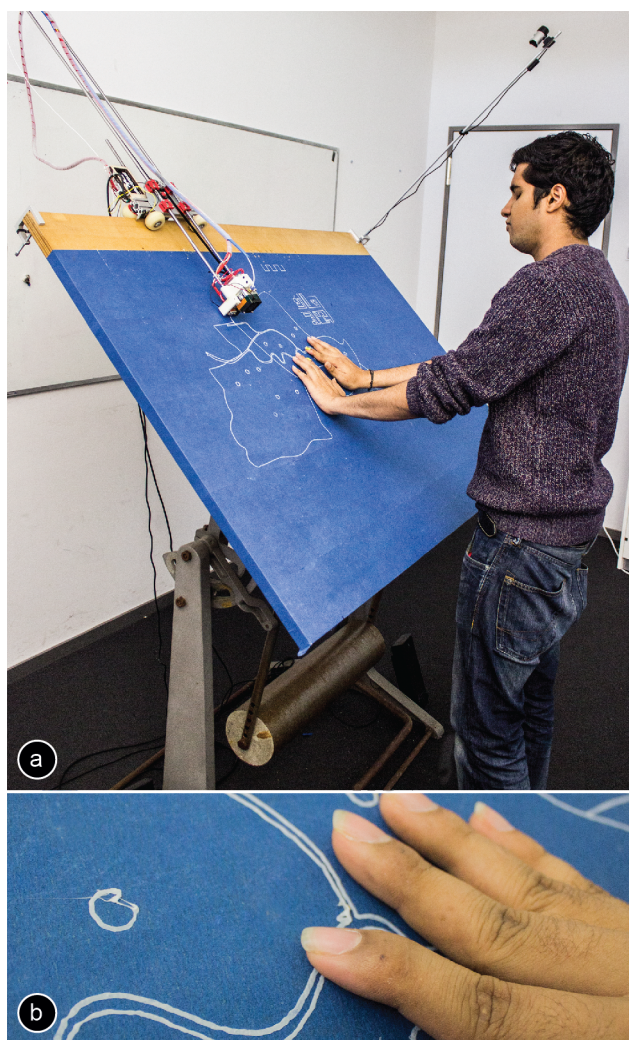
Figure 1: (a) Linespace is a sensemaking platform for the blind. Its custom display hardware offers 140 x 100cm display space and it draws lines as its main primitive. Here Linespace runs the home-finder application that enables users to browse maps in search for a home. (b) Linespace's main primitive is raised lines, which it produces using a modified 3D printer.
