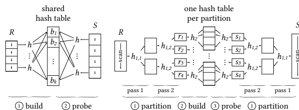
Figure 1: No partitioning join
