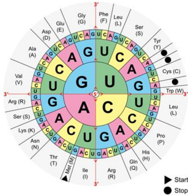
FIGURE 6 RNA Codons and how they translate into amino acids. One letter code of amino acids is given in brackets.
