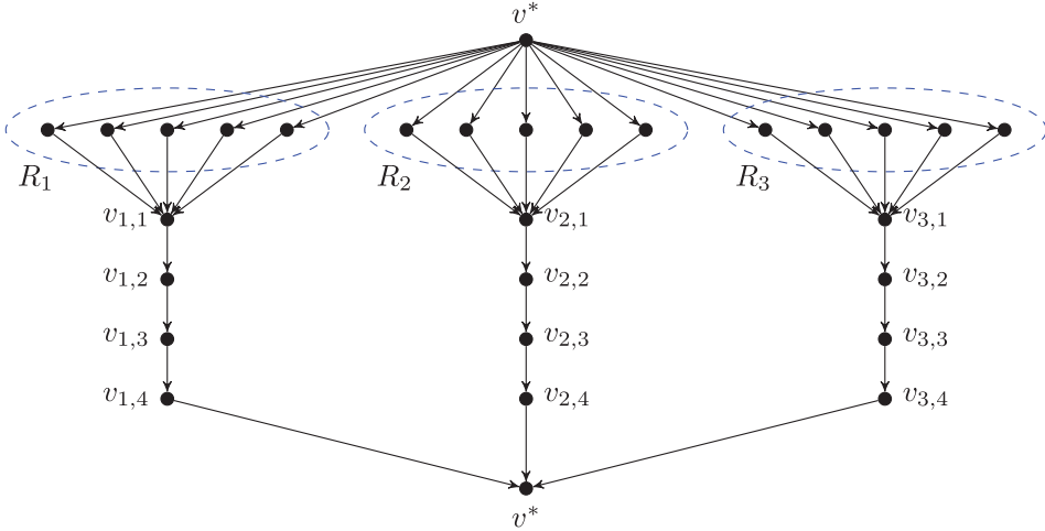
Fig. 2. The superstar \mathcal{S}_{4,3,5} , with \ell = 3 reservoirs R_1 , R_2 , and R_3 , each of size m = 5 , connected by a path with k = 4 vertices to v^* . The centre vertex v^* is shown twice, at both the top and bottom of the diagram.
