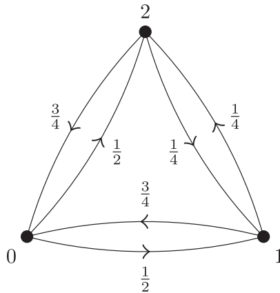
Fig. 4. A three-vertex graph which is not isothermal but has fixation probability \rho_{\text{reg}}(r, 3) .
