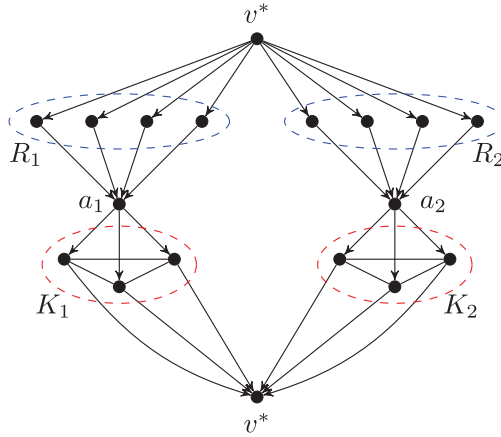
Fig. 3. The megastar \mathcal{M}_{3,2,4} , with \ell = 2 reservoirs R_1 and R_2 , each of size m = 4 . Each reservoir R_i is attached, via the feeder vertex a_i , to a clique of size k = 3 . The centre vertex v^* is shown twice, once at the top and once at the bottom of the diagram. The edges within the cliques K_1 and K_2 are bidirectional.
