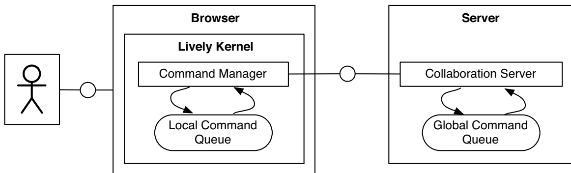
Fig. 2: High-level architecture of collaboration framework
