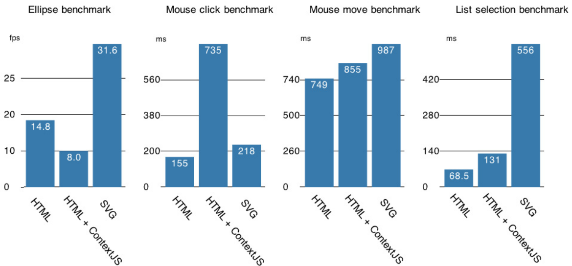
Fig. 6: Results of the benchmark comparing the performance of the HTML and SVG version.
