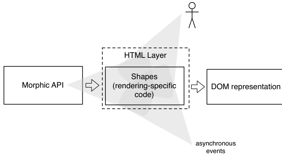
Fig. 3: Locations for layered code and the different types of layer activation
