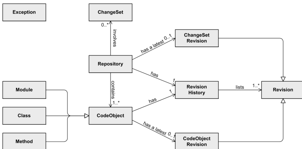
Fig. 2: Code Database API: Class Diagram
