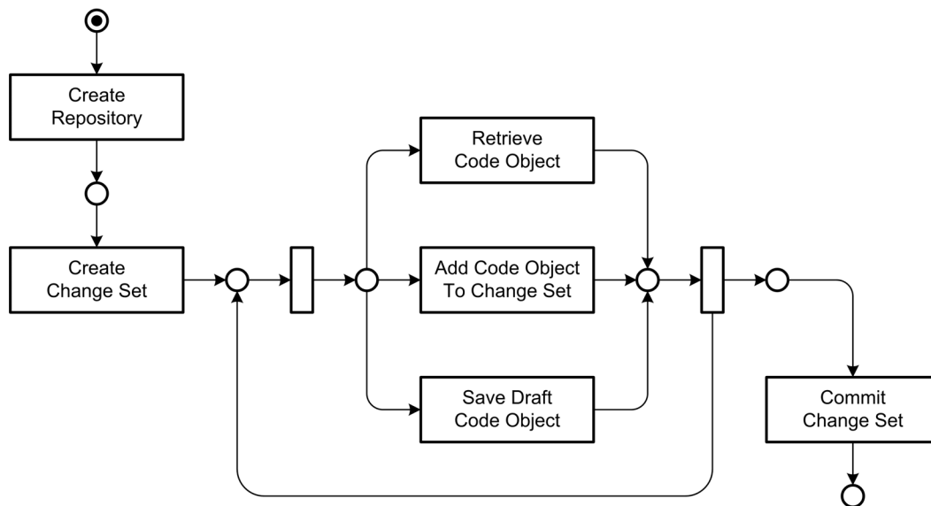
Fig. 3: Typical Program Flow
