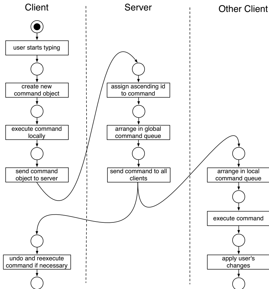
Fig. 1: Command life cycle using the example of an user who is typing text
