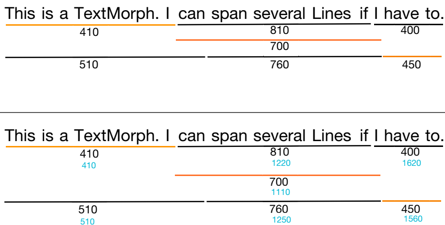
Fig. 2: Simplified intermediate result of the KPA. Above: Five possible breakpoints were found. The cost of the lines each breakpoint creates is given. Below: Additional to the previous, the accumulated cost from the beginning of the paragraph is given. The highlight sequence denotes the sequence of chosen breakpoints.
