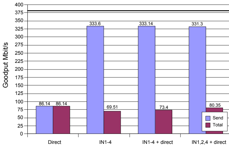
Figure 6 Experimental results using 4*100 Mbit lines.
