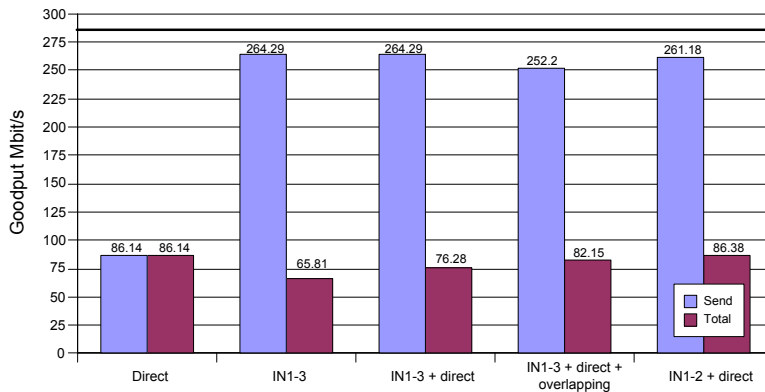
Figure 5 Experimental results using 3*100 Mbit lines.
